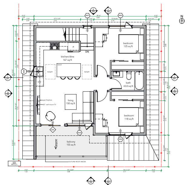
1 D3 Suite Level SCALE: 3/16" = 1'-0"
